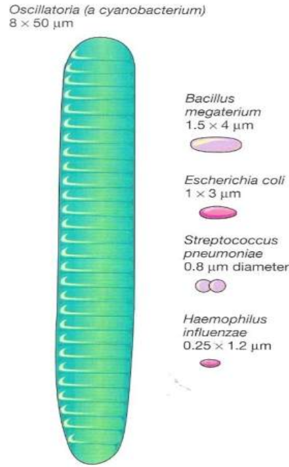
FIGURE 3.14 Comparison of sizes of a variety of prokaryotes. Most known prokaryotes have cell diameters in the range of 0.5–2 μm.
